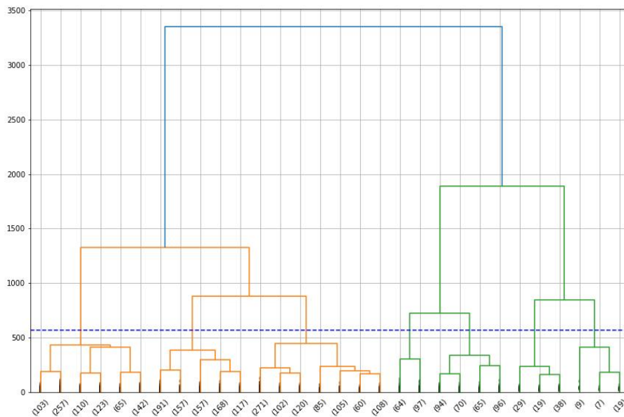
Figure 3.28: Dendrogram
