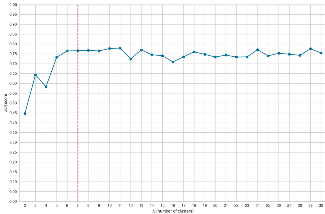
Figure 3.34: GDI Score
