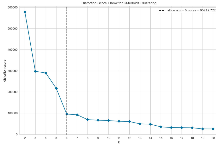
Figure 3.45: Elbow curve
