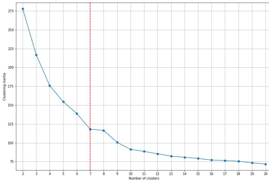
Figure 3.26: Elbow curve
