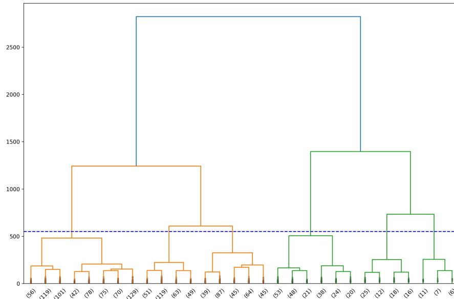
Figure 3.20: Dendrogram
