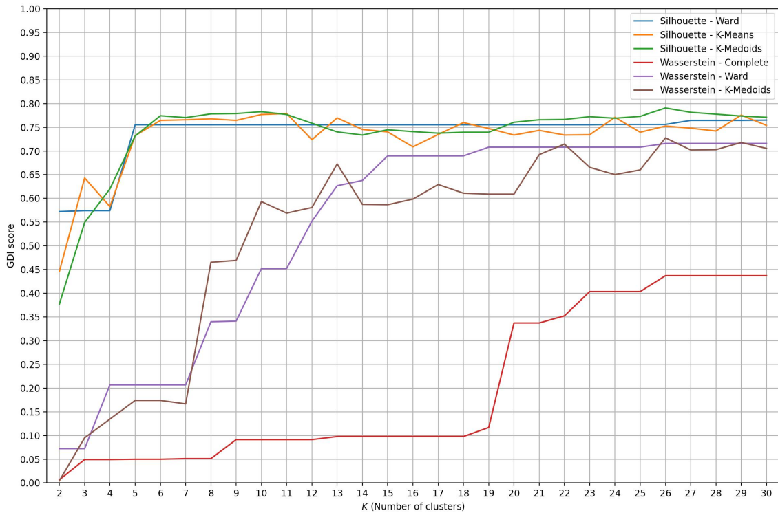
Figure 3.37: GDI Score - Overview
