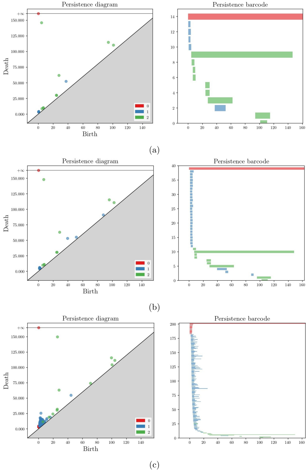
Figure 3.5: (a) Original point set (b) ASAP subsample and (c) random subsample.
