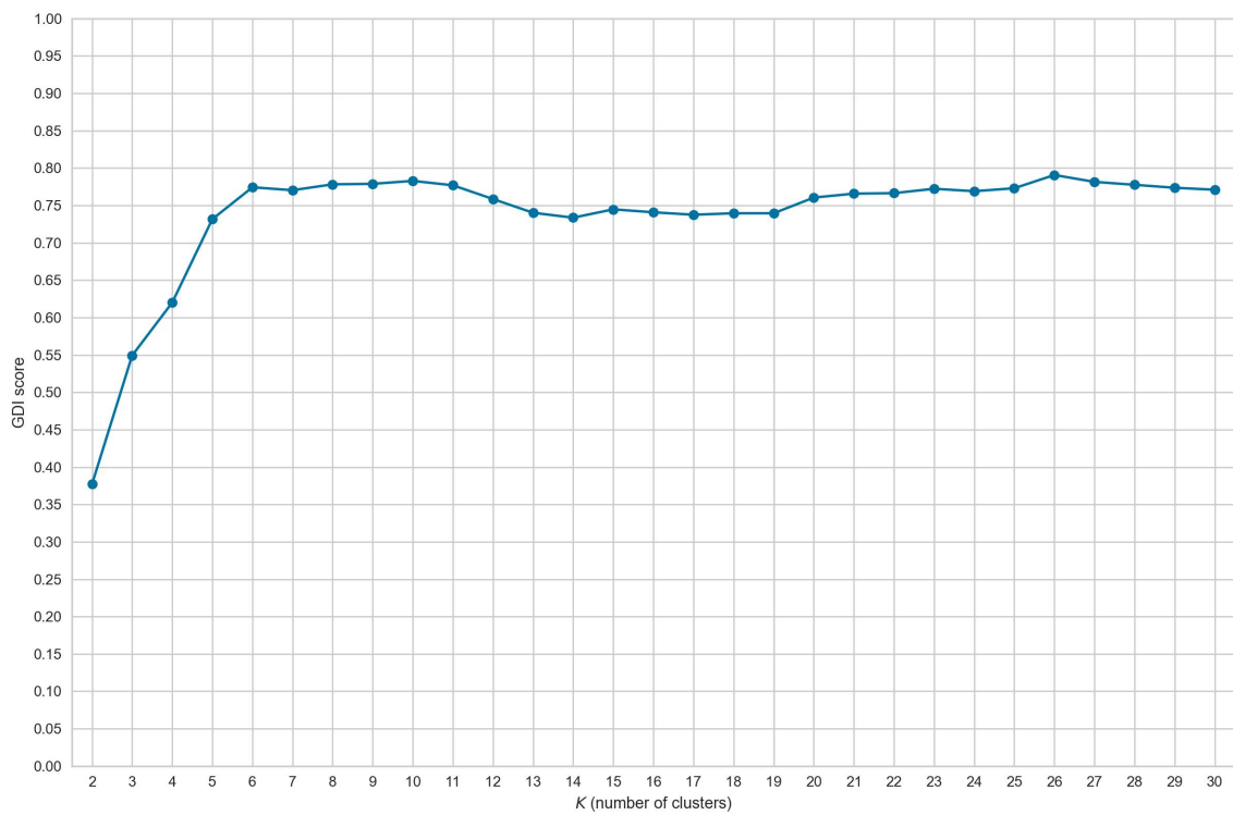
Figure 3.36: GDI Score
