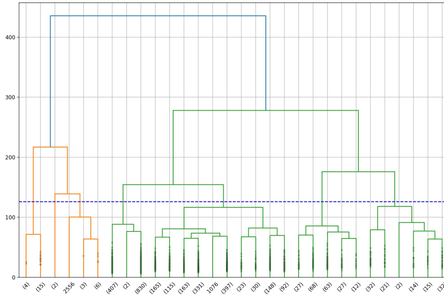
Figure 3.25: Dendrogram
