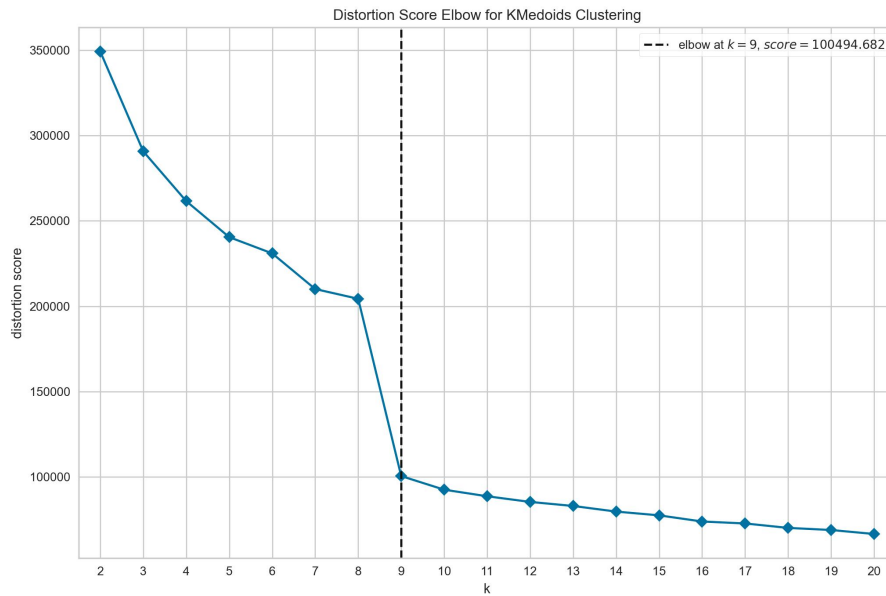
Figure 3.47: Elbow curve
