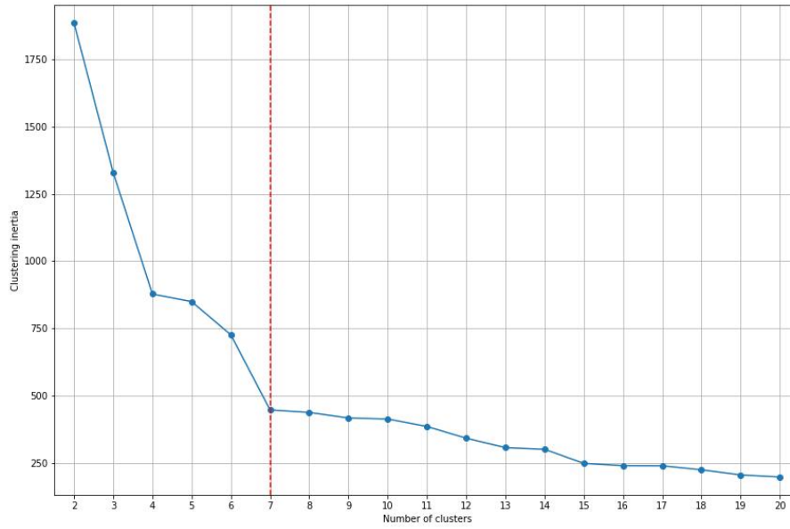
Figure 3.29: Elbow curve
