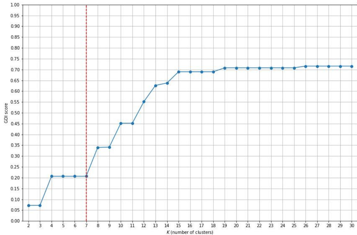
Figure 3.30: Evolution of the GDI score as a function of the number of K clusters.
