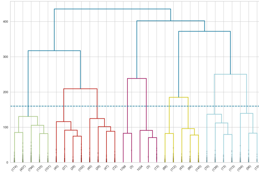
Figure 3.31: Dendrogram
