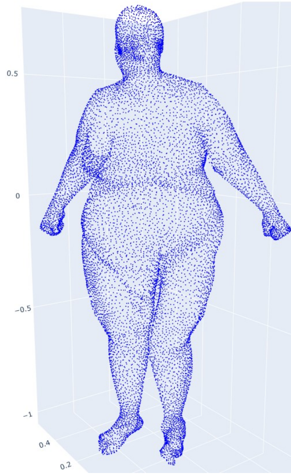
Figure 3.38: S_{init}
