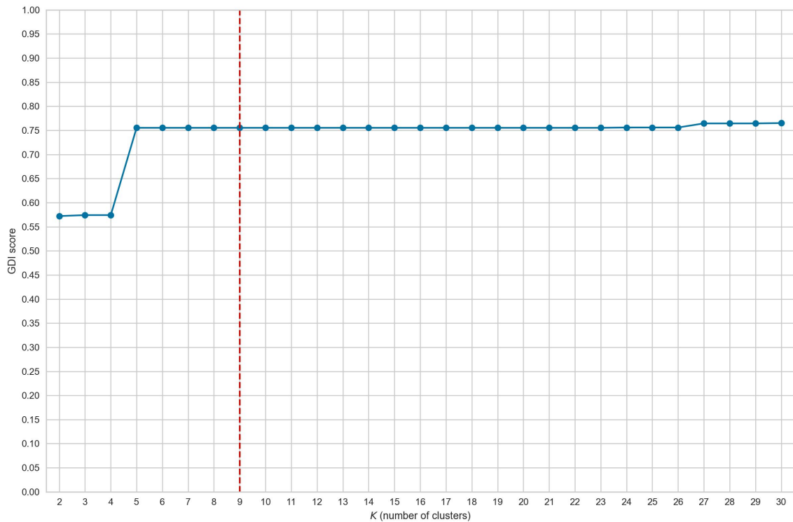
Figure 3.32: GDI Score
