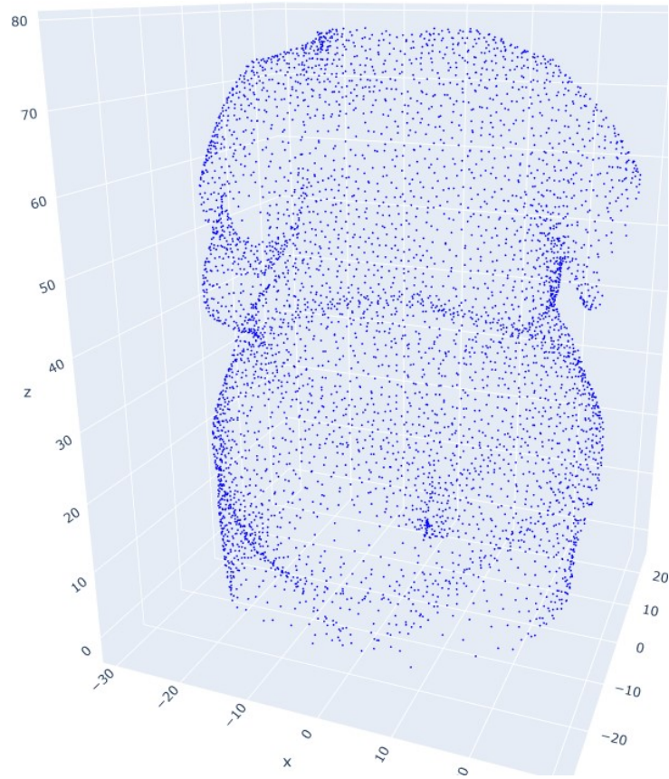
Figure 3.42: S_{final}
